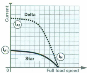
Typical speed/current curve
