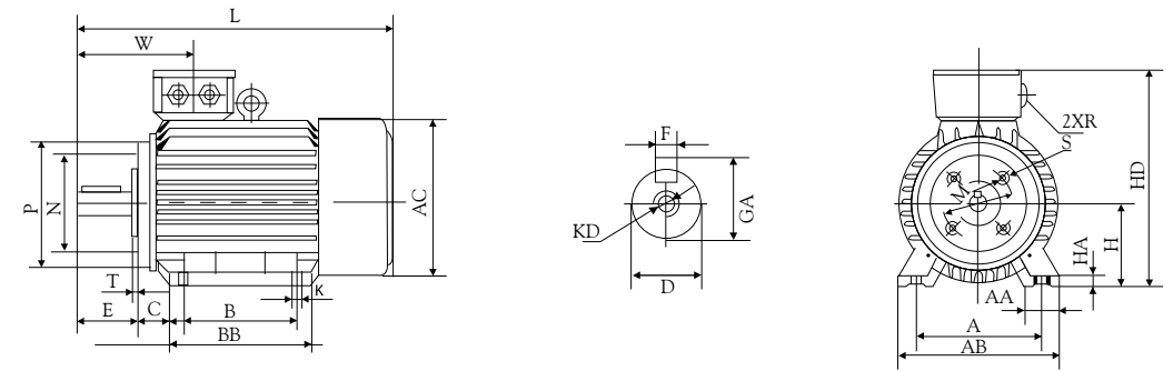
B3/B14-Foot/Face mounting
