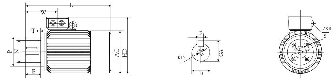
B14-Face mounting
